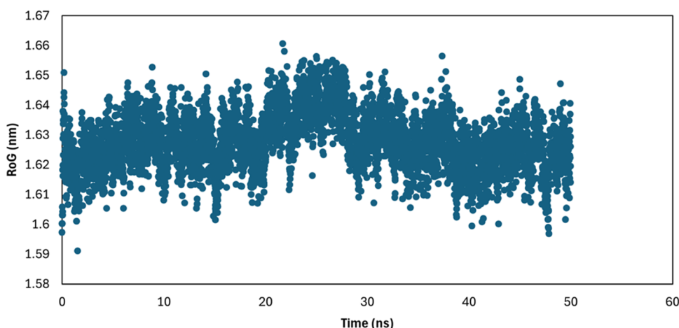
Figure 8. RoG stabilization indicates compactness of the ternary complex.
