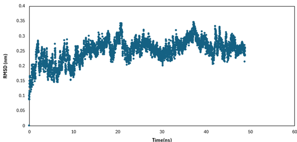
Figure 7. RMSD stabilization indicates the stability of the ternary complex.
